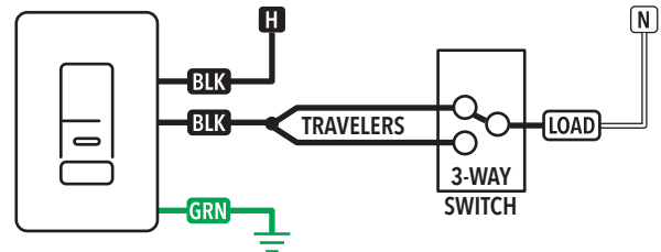
3-way switch does not influence LOAD status
