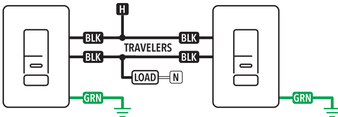
Both sensors required to time out to switch LOAD off
